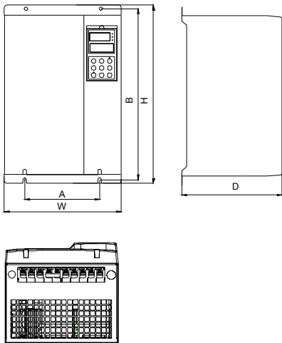
图2-3 TD3100-4T0185E~TD3100-4T0300E
